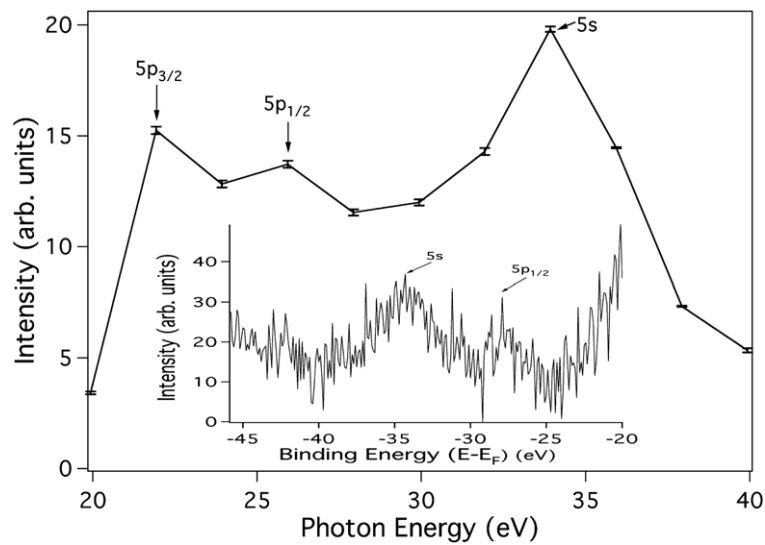
Figure 3. The photoemission intensities at 6 eV binding energy for Gd@C 60 , as a function of photon energy. The photoemission intensities are seen to increase at photon energies that roughly correspond to the Gd 5s and 5p shallow core edges, indicating a resonant photoemission process that includes Gd. In the inset, a photoemission spectrum, taken at higher photon energy, 95 eV, indicates the binding energies of the Gd 5s and 5p 1/2 cores in Gd@C 60 .
